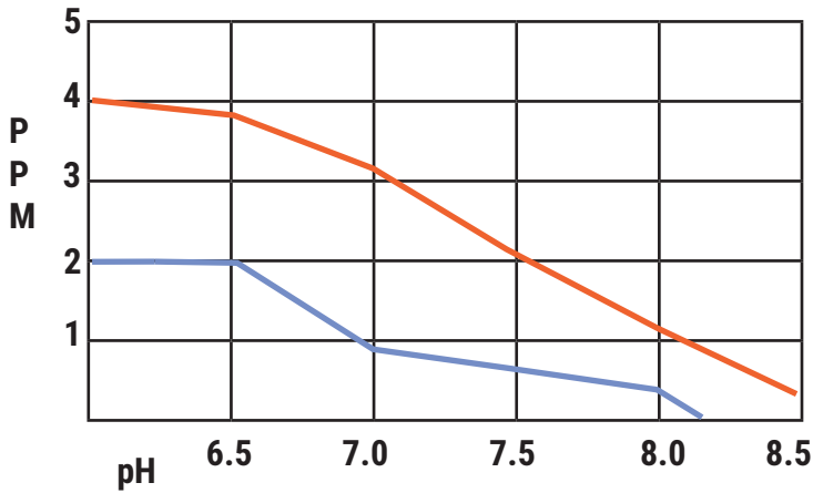
Sulfur Removal Capacity
